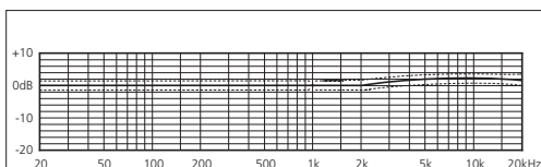
Frequency response curve CCM 5 "omni" position Polar diagram as CCM 2, -2H, -2S, -3
