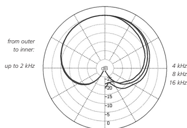
Polar diagram CCM 5
