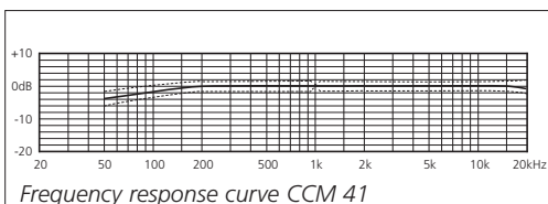
Frequency response curve CCM 41
