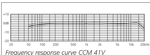
Frequency response curve CCM 41V
