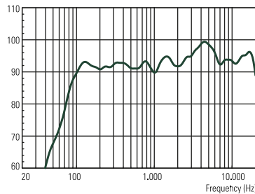
RESPONSE 1W/1m
