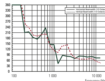
BEAMWIDTH vs. FREQUENCY
