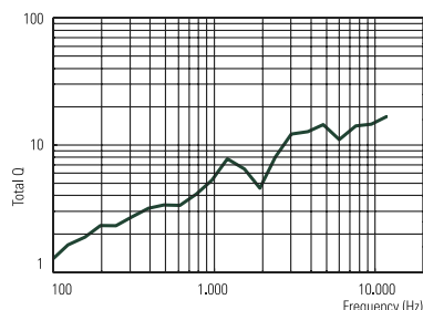
DIRECTIVITY INDEX AND Q
