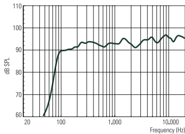
RESPONSE 1W/1m
