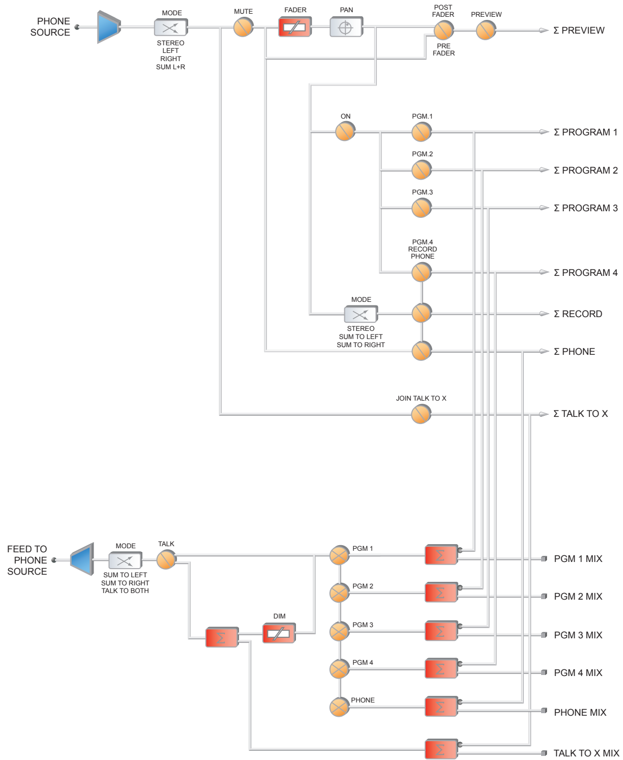
Figure B-4 Block Diagram - Phone Source
