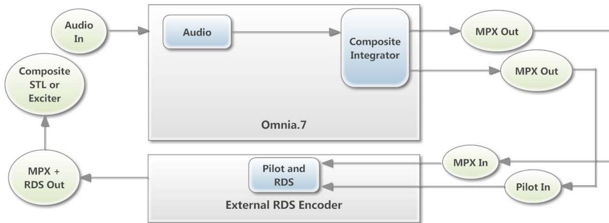
RDS Using External Encoder After Omnia.7
