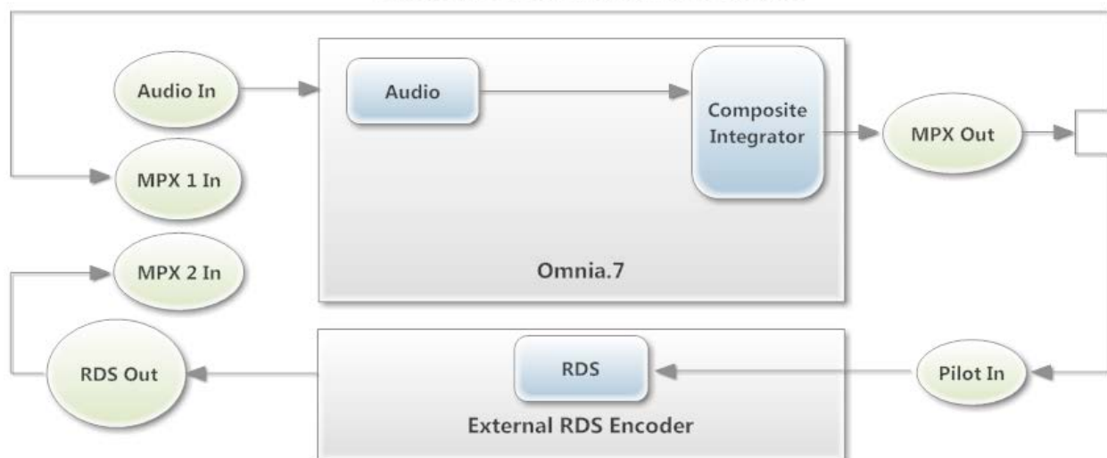
RDS Using External Encoder That Does Not Provide a Pilot Signal After Omnia.7
